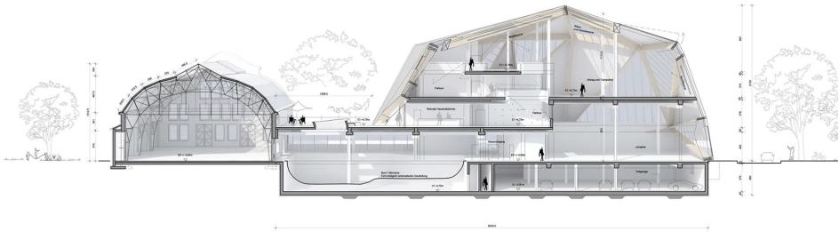
Section
