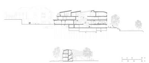
Section AA, BB
