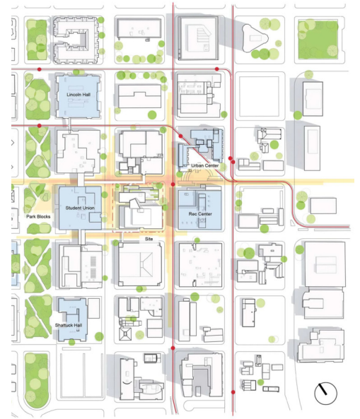
Site Plan
