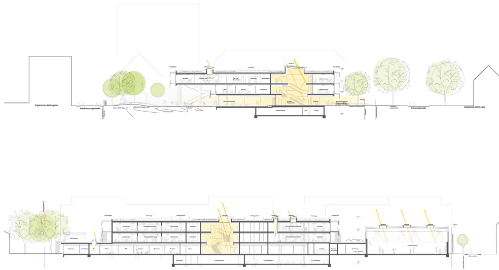
Section AA & BB
