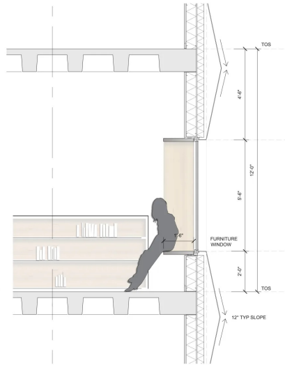
Facade Details
