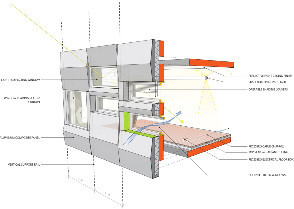
Facade Detail
